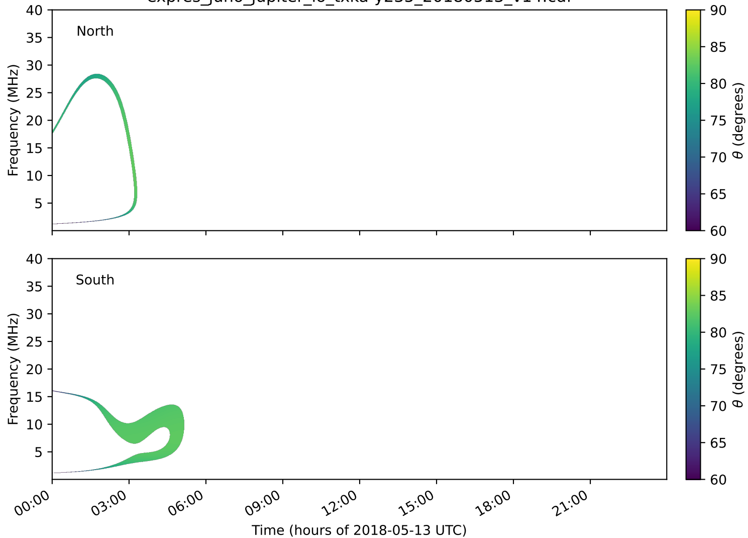
expres_juno_jupiter_io_txka-y235_20180513_v14.cdf
