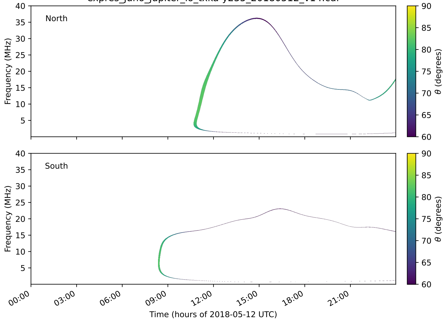
expres_juno_jupiter_io_txka-y235_20180512_v14.cdf
