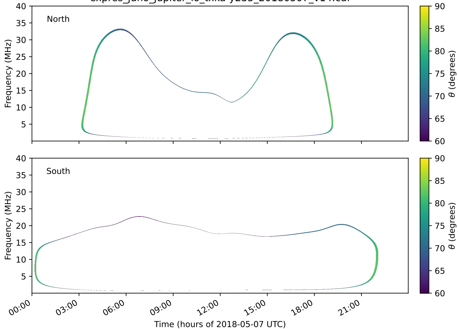
expres_juno_jupiter_io_txka-y235_20180507_v14.cdf
