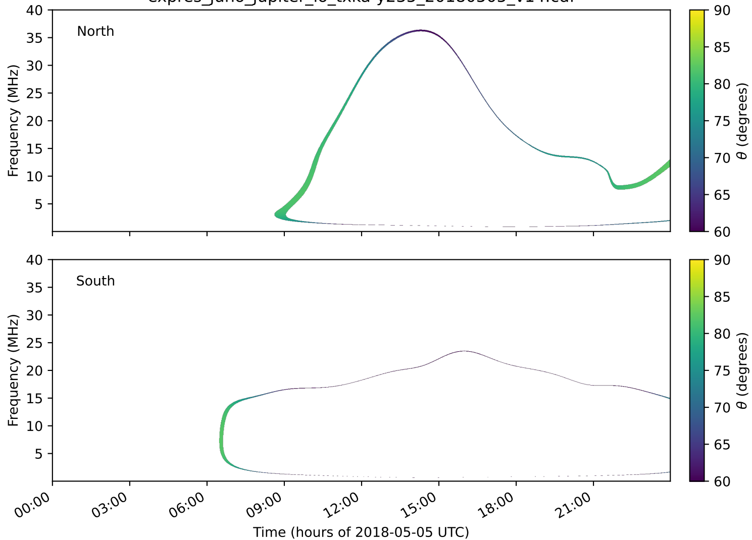
expres_juno_jupiter_io_txka-y235_20180505_v14.cdf
