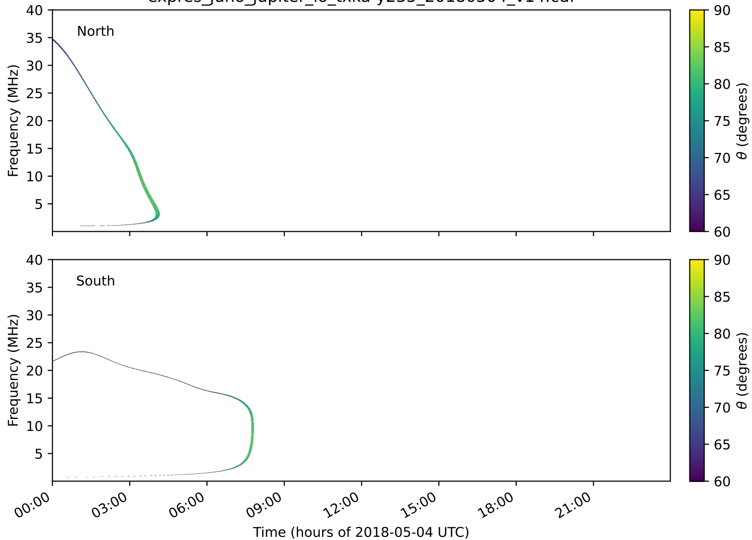
expres_juno_jupiter_io_txka-y235_20180504_v14.cdf
