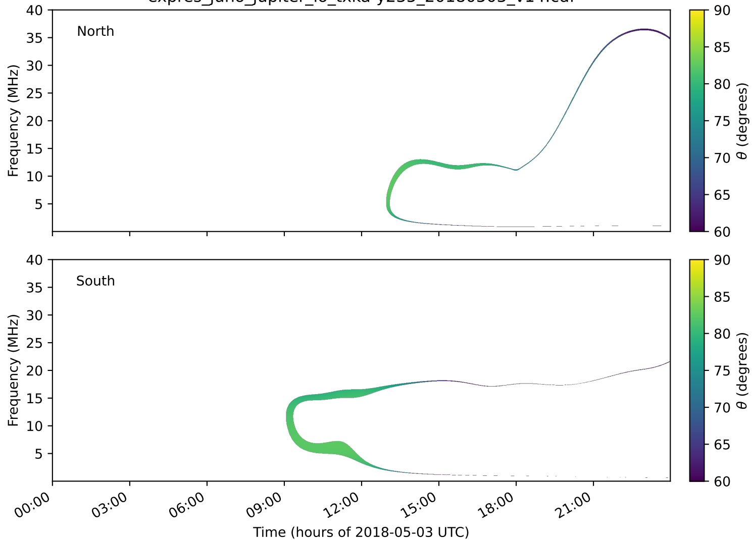
expres_juno_jupiter_io_txka-y235_20180503_v14.cdf
