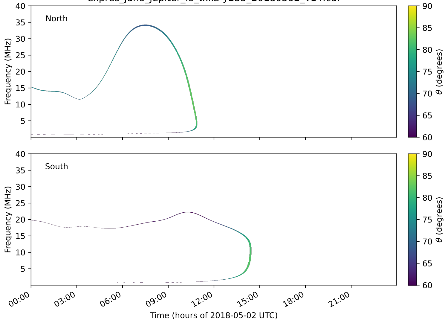
expres_juno_jupiter_io_txka-y235_20180502_v14.cdf
