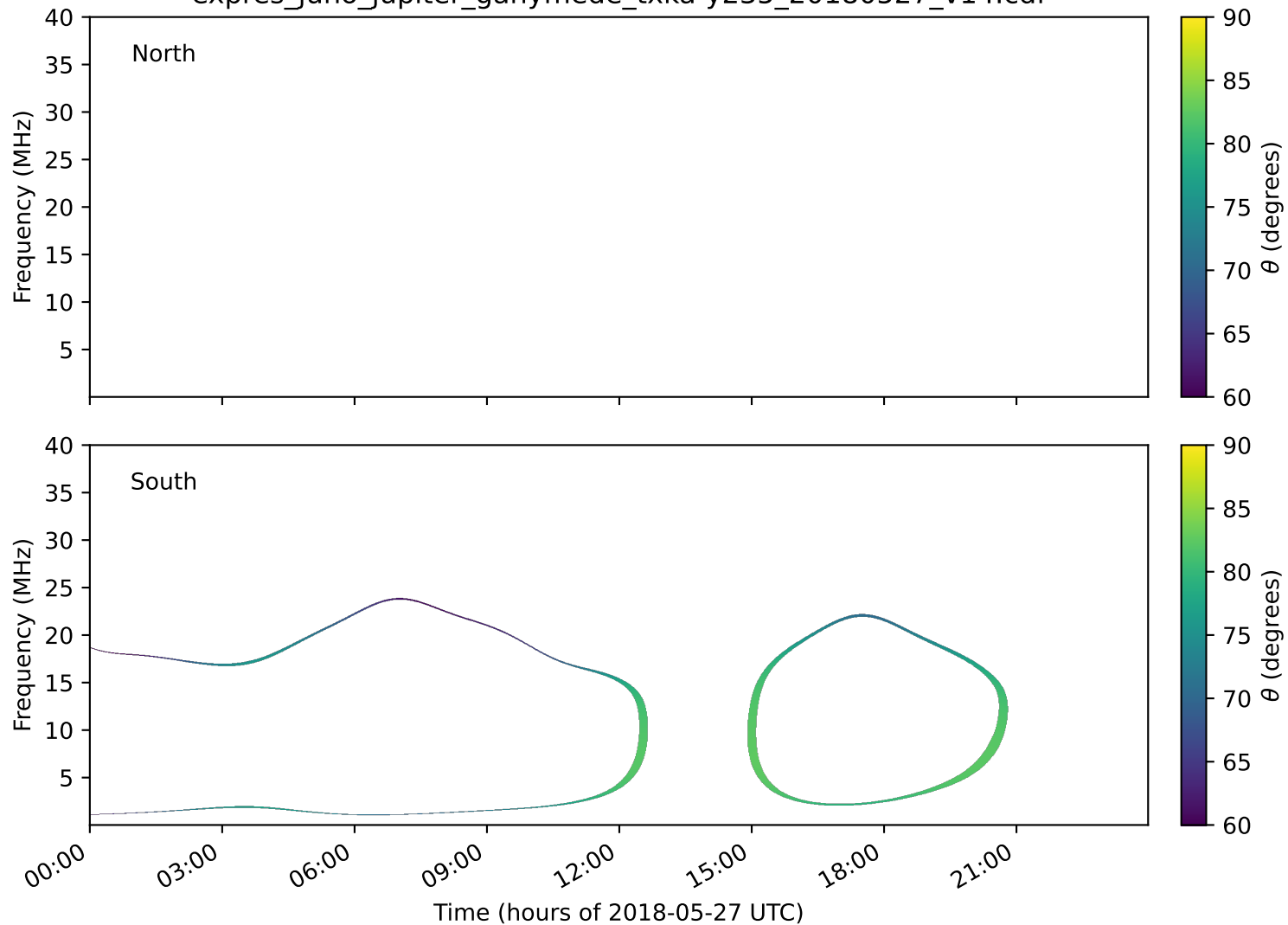
expres_juno_jupiter_ganymede_txka-y235_20180527_v14.cdf
