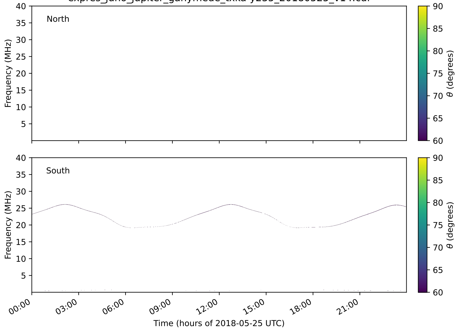
expres_juno_jupiter_ganymede_txka-y235_20180525_v14.cdf
