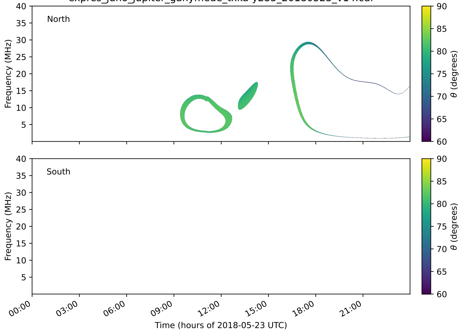
expres_juno_jupiter_ganymede_txka-y235_20180523_v14.cdf
