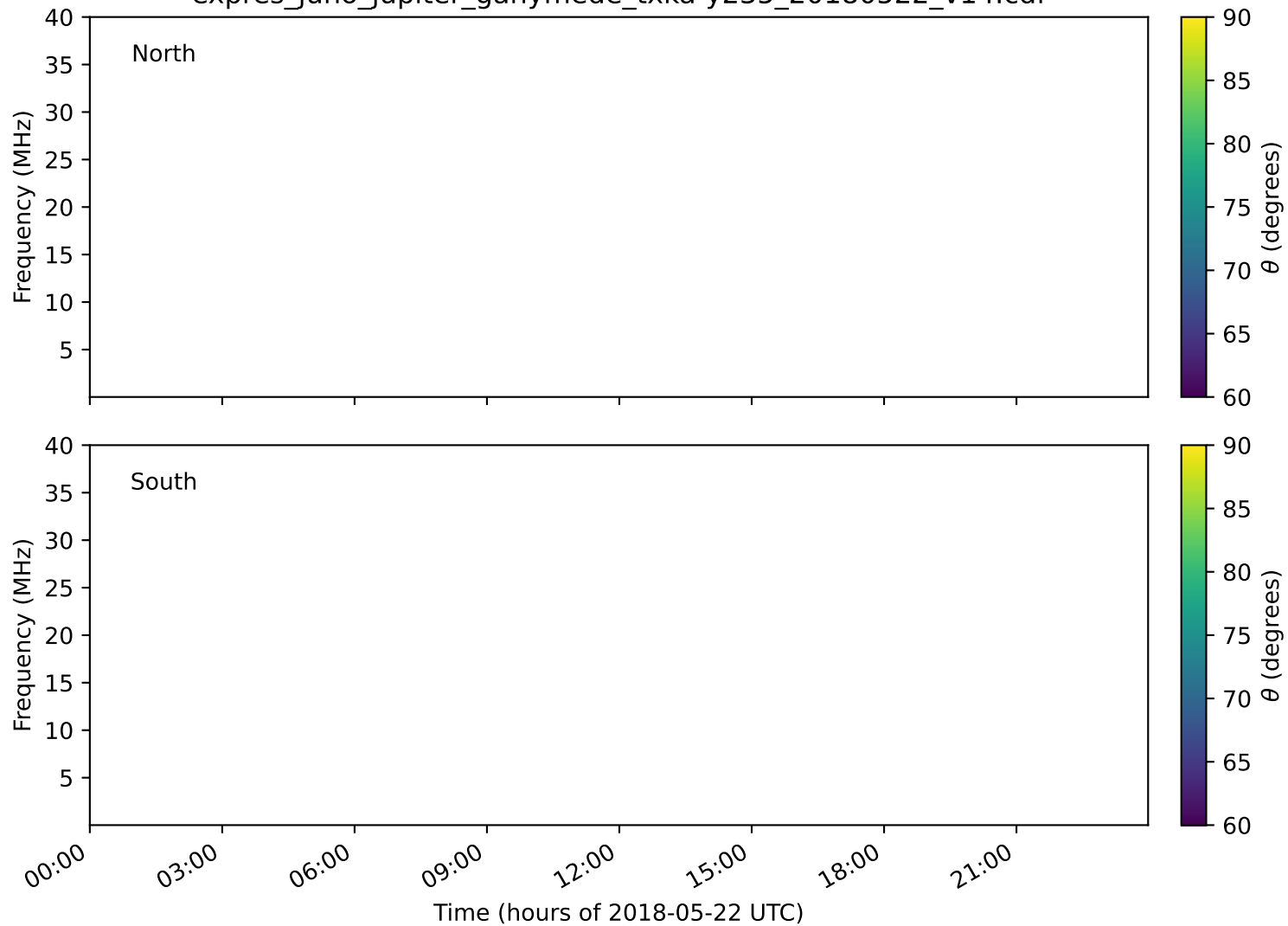
expres_juno_jupiter_ganymede_txka-y235_20180522_v14.cdf
