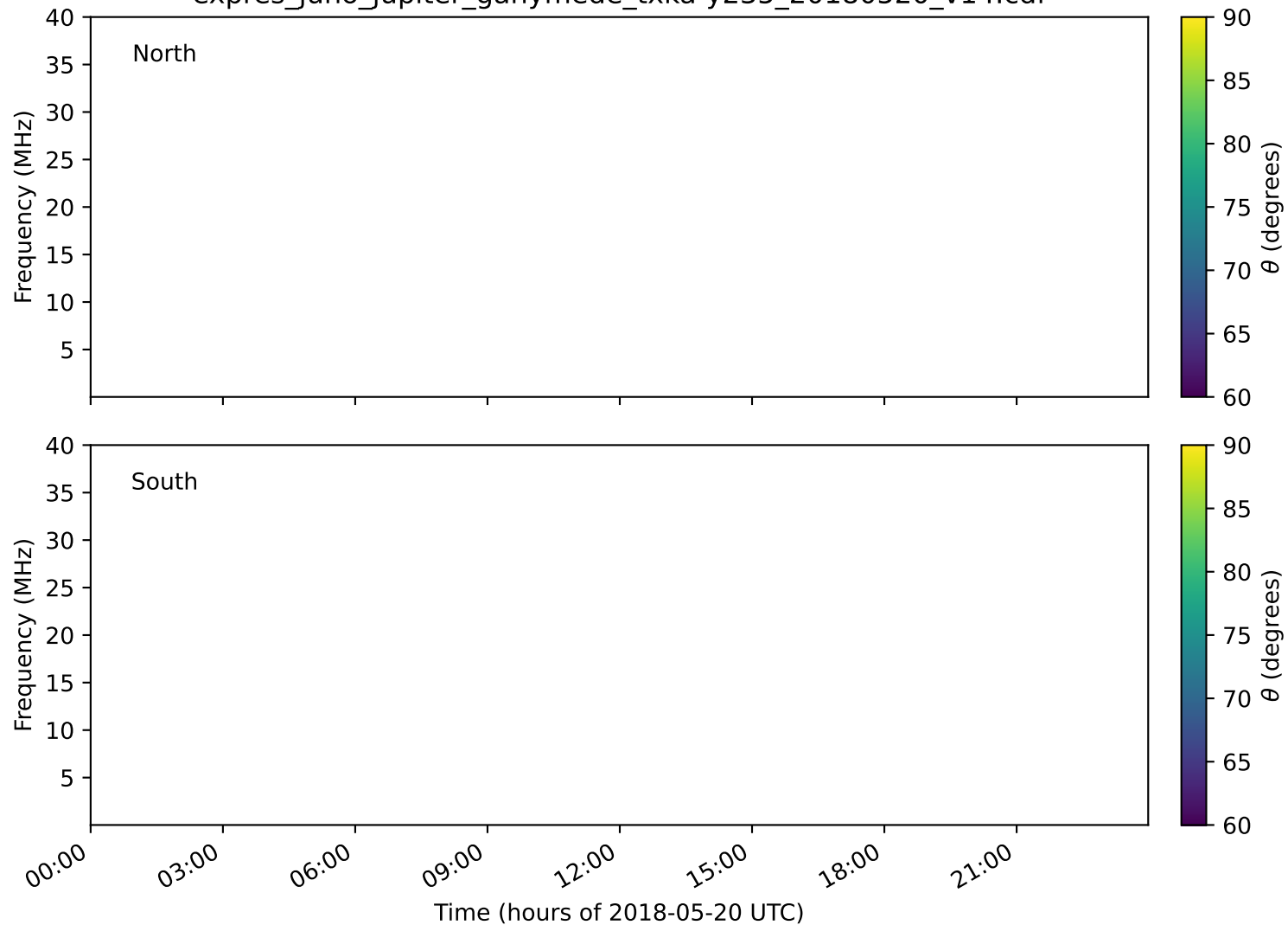
expres_juno_jupiter_ganymede_txka-y235_20180520_v14.cdf
