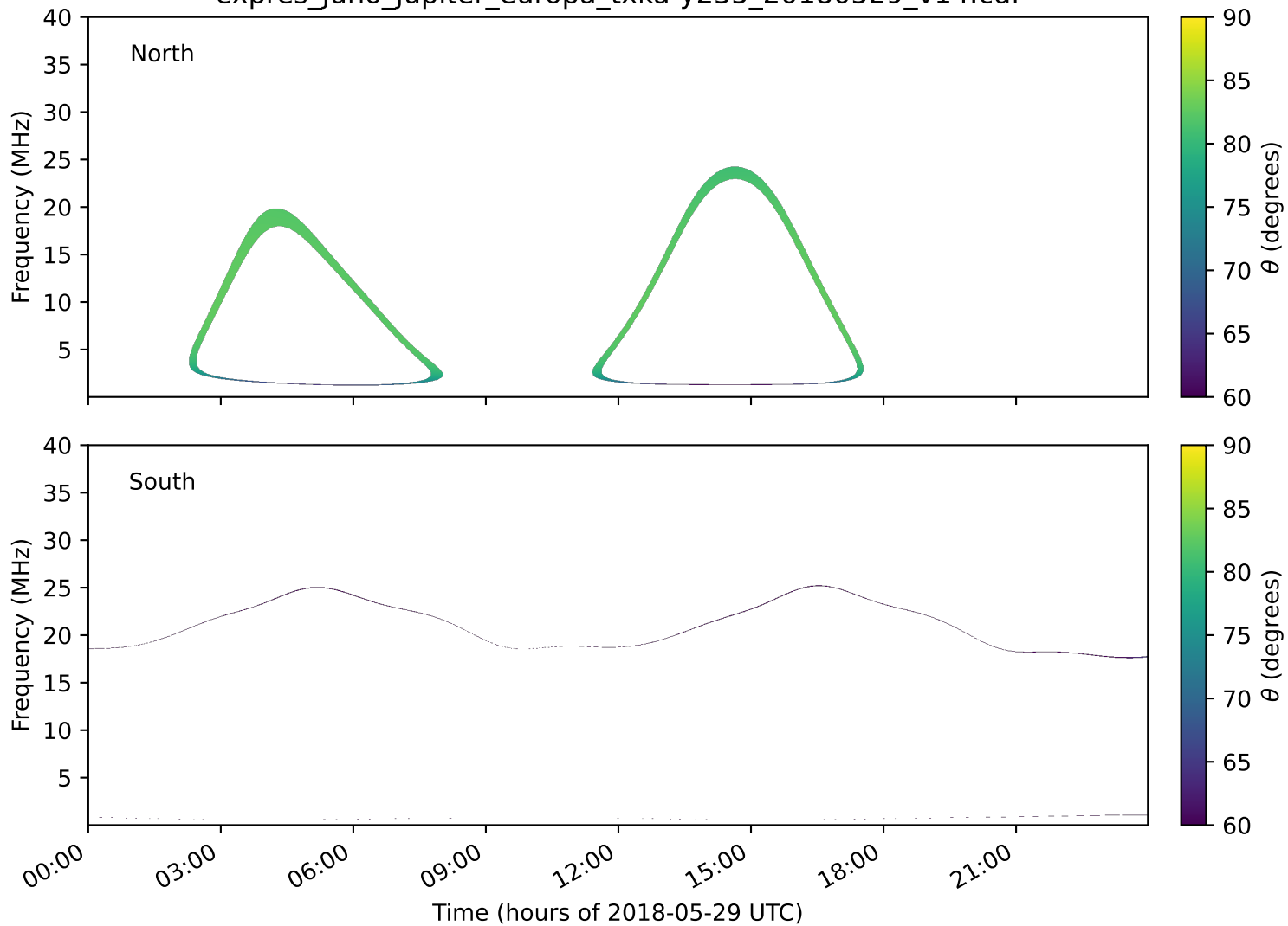
expres_juno_jupiter_europa_txka-y235_20180529_v14.cdf
