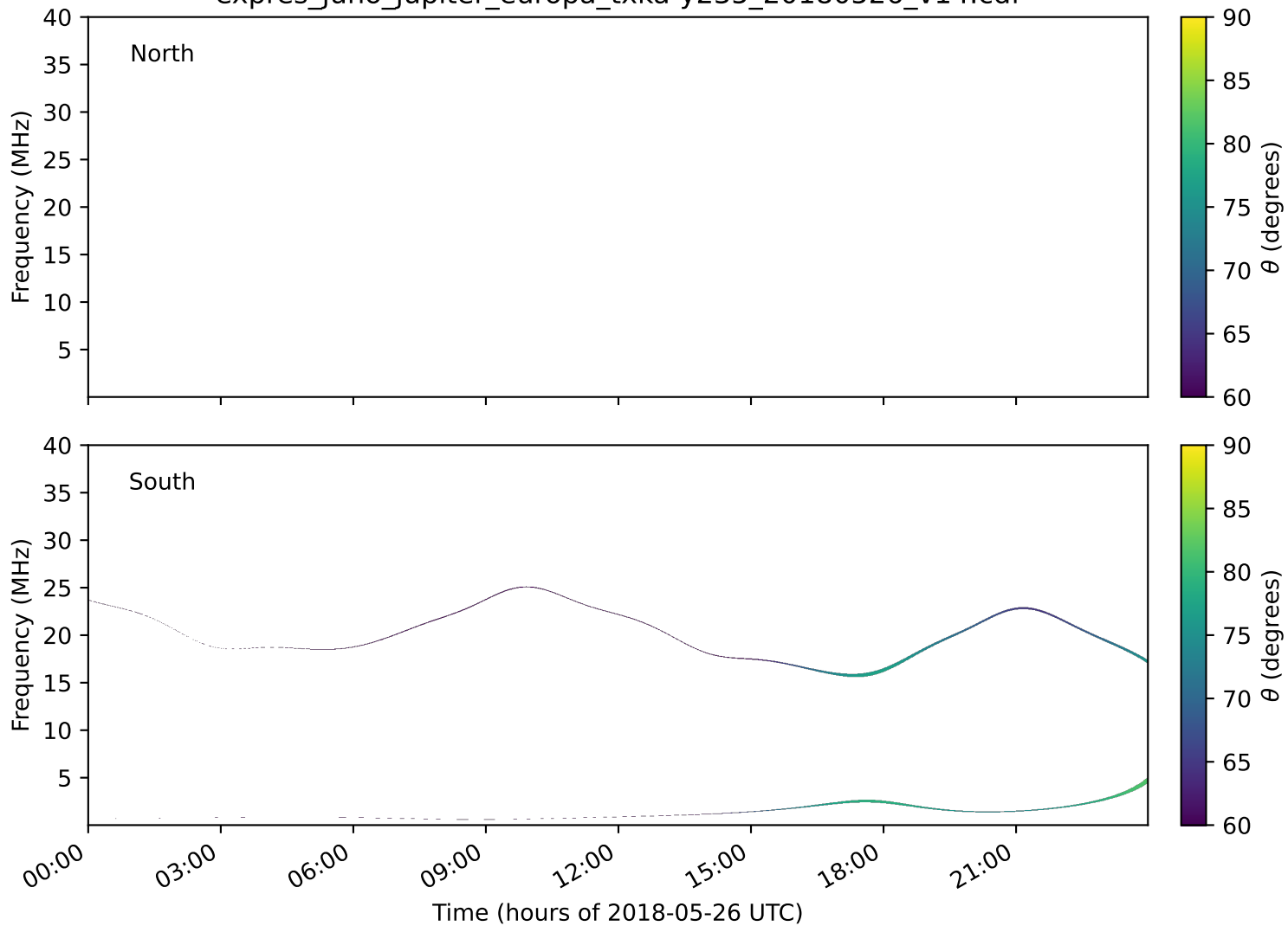
expres_juno_jupiter_europa_txka-y235_20180526_v14.cdf
