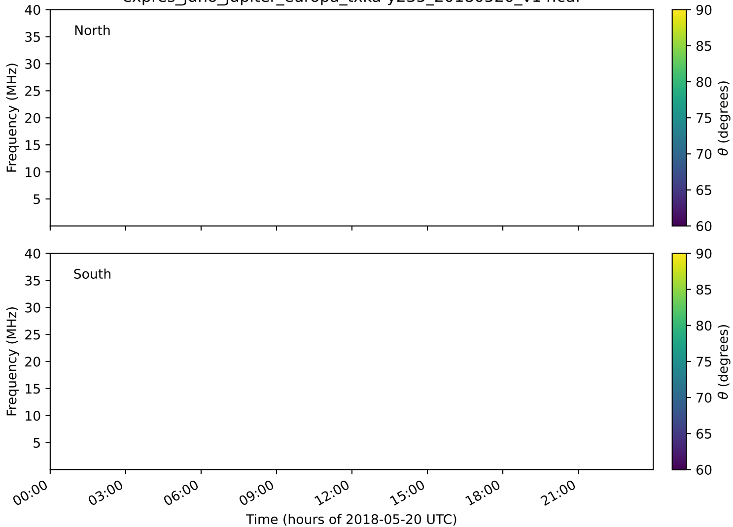
expres_juno_jupiter_europa_txka-y235_20180520_v14.cdf
