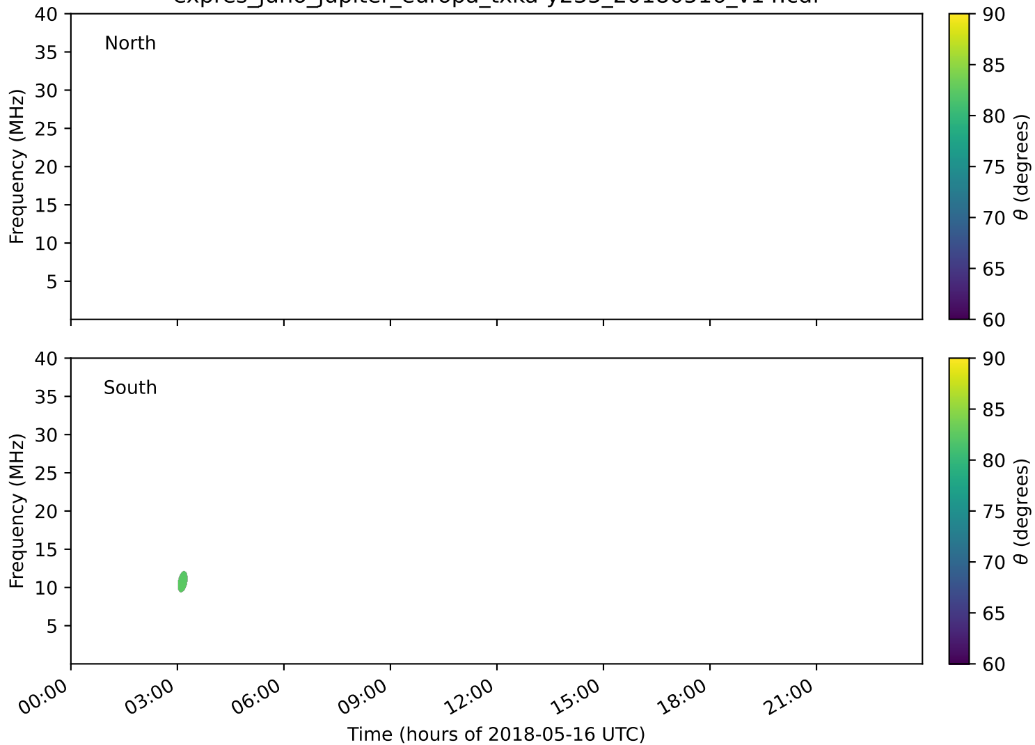
expres_juno_jupiter_europa_txka-y235_20180516_v14.cdf
