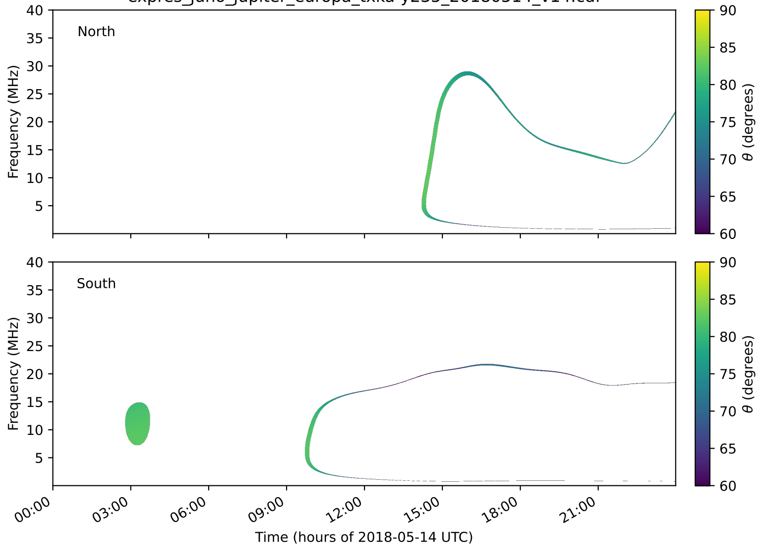
expres_juno_jupiter_europa_txka-y235_20180514_v14.cdf
