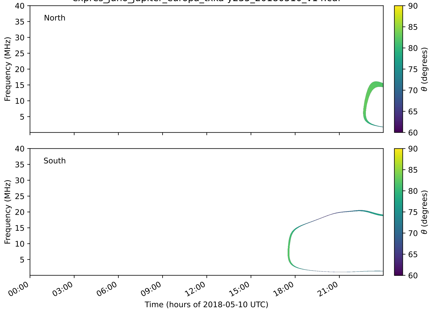
expres_juno_jupiter_europa_txka-y235_20180510_v14.cdf
