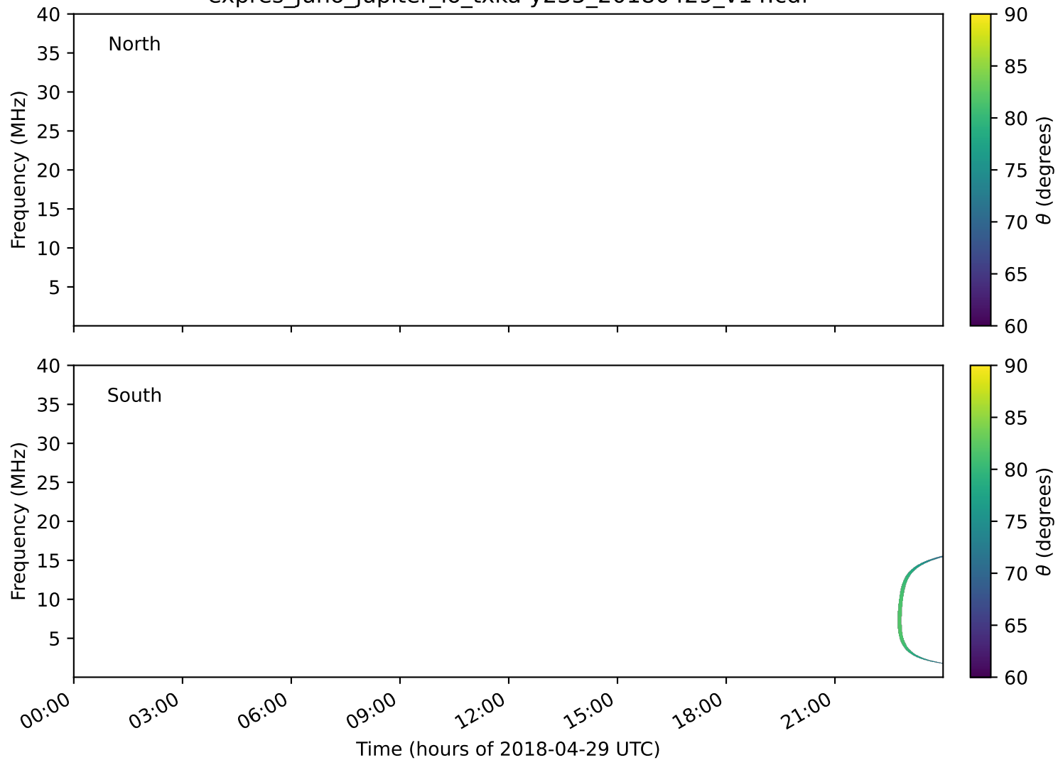
expres_juno_jupiter_io_txka-y235_20180429_v14.cdf
