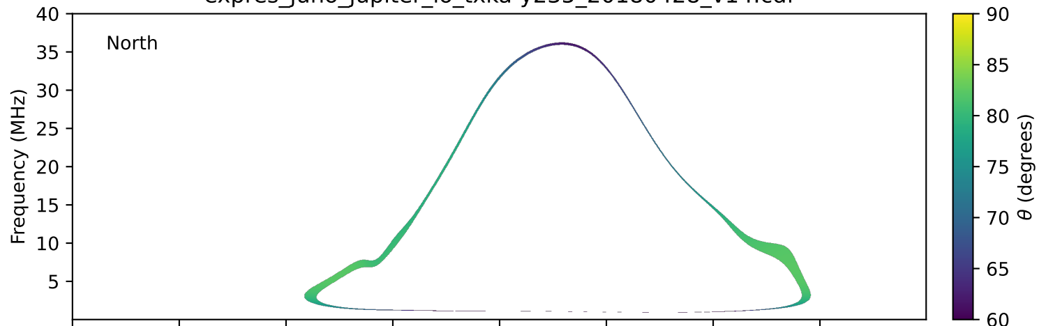
expres_juno_jupiter_io_txka-y235_20180428_v14.cdf
