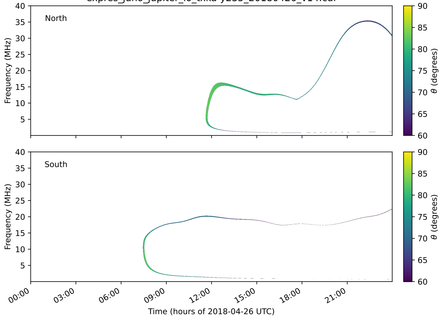
expres_juno_jupiter_io_txka-y235_20180426_v14.cdf
