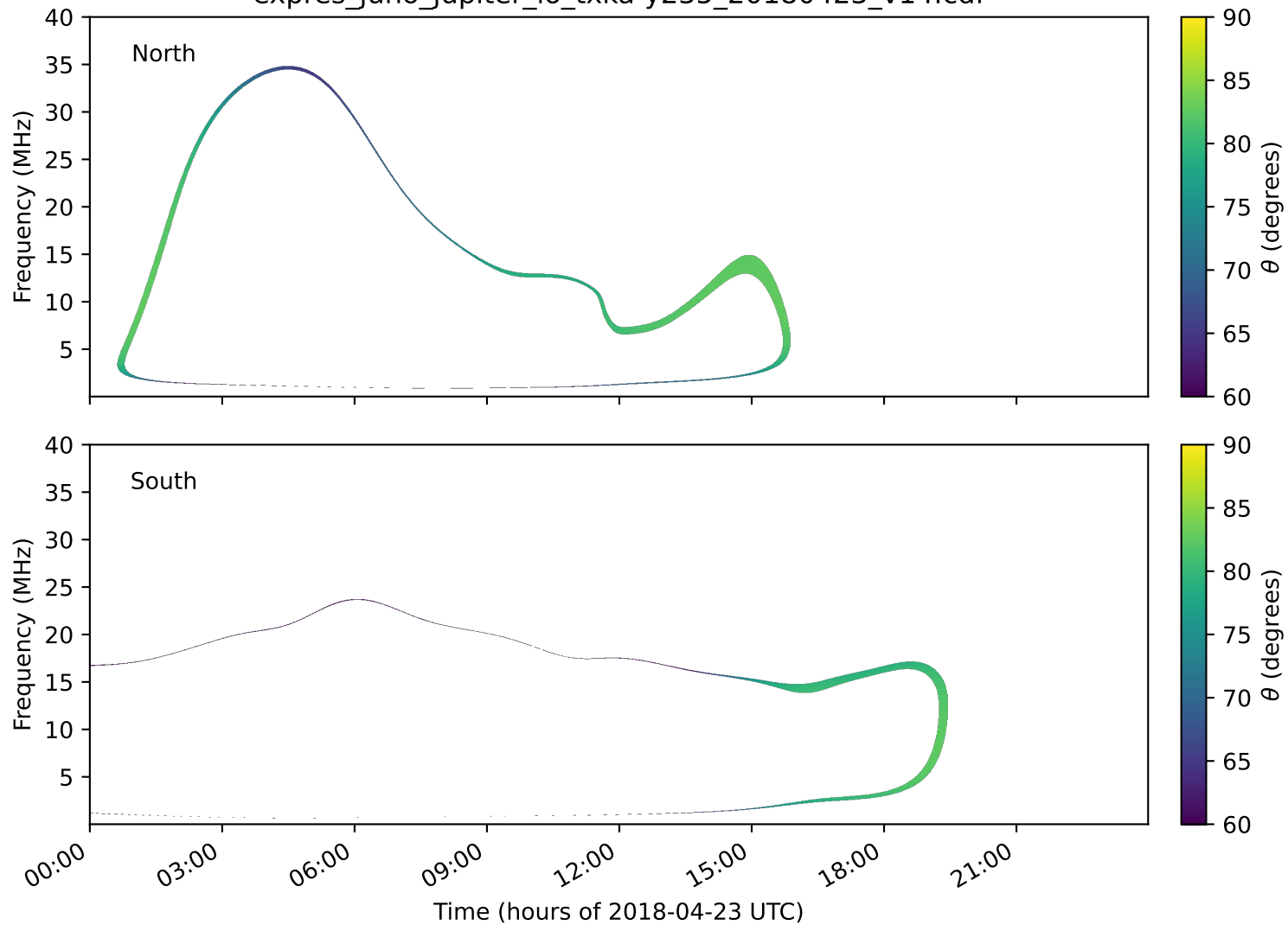
expres_juno_jupiter_io_txka-y235_20180423_v14.cdf
