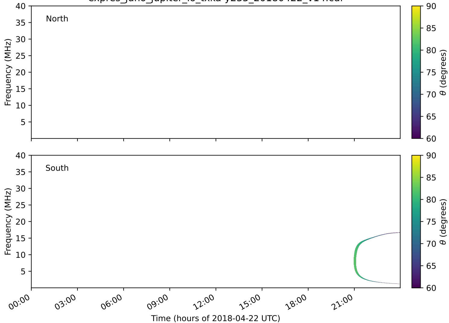
expres_juno_jupiter_io_txka-y235_20180422_v14.cdf
