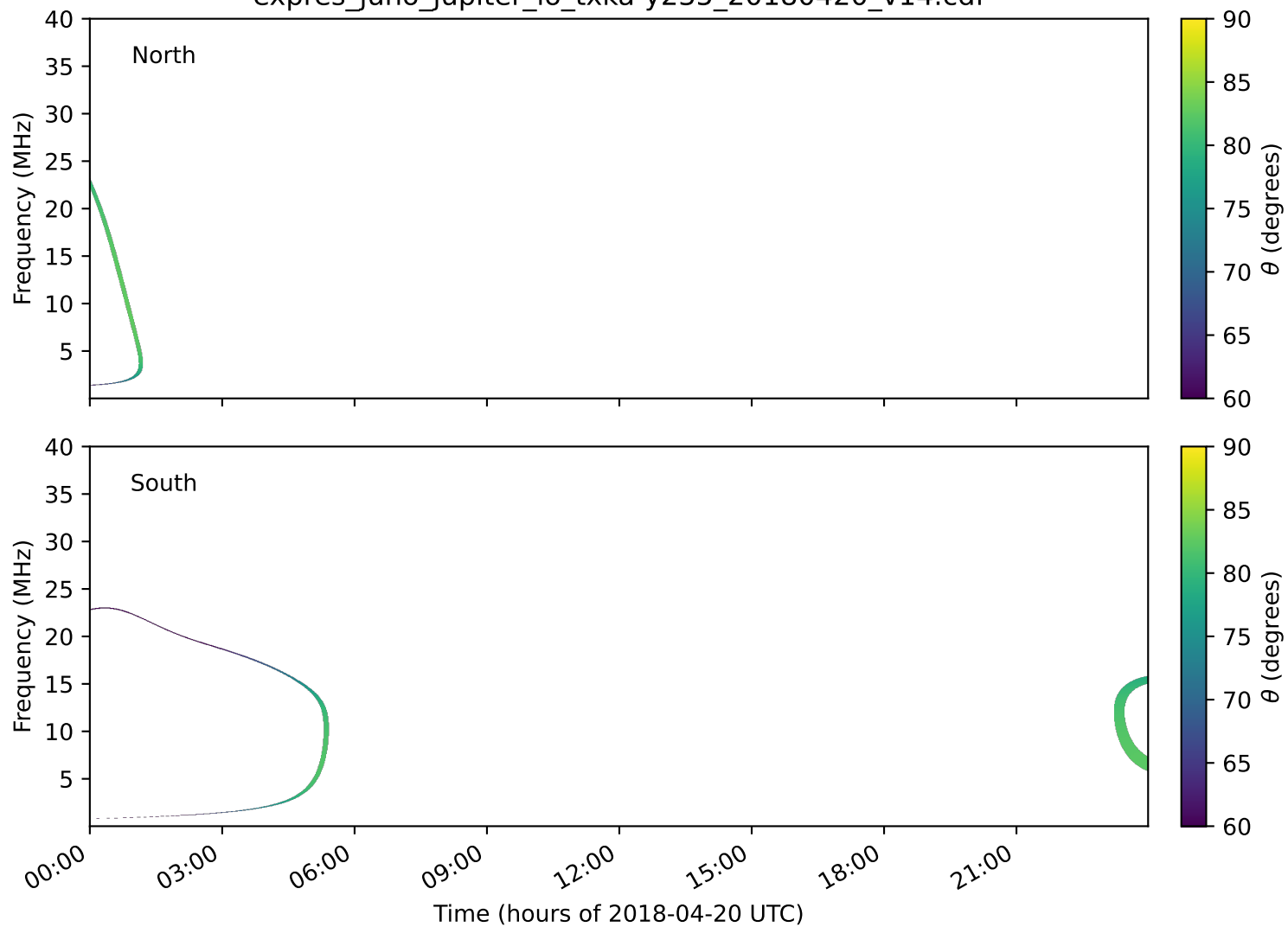
expres_juno_jupiter_io_txka-y235_20180420_v14.cdf
