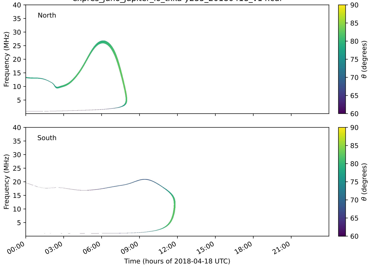
expres_juno_jupiter_io_txka-y235_20180418_v14.cdf
