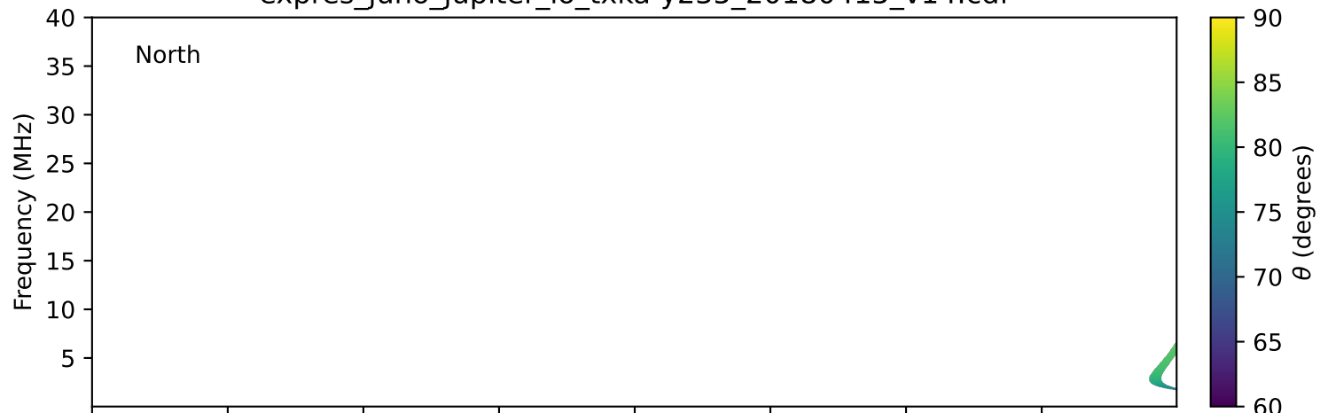
expres_juno_jupiter_io_txka-y235_20180415_v14.cdf
