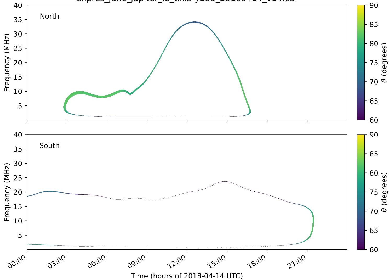
expres_juno_jupiter_io_txka-y235_20180414_v14.cdf
