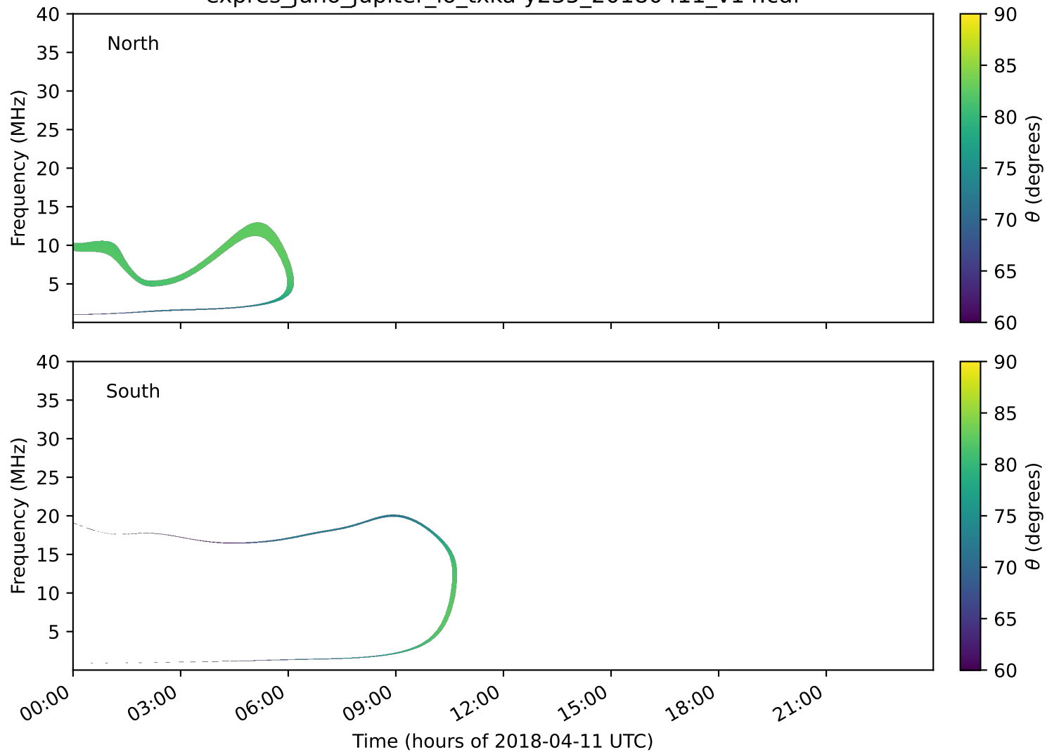
expres_juno_jupiter_io_txka-y235_20180411_v14.cdf
