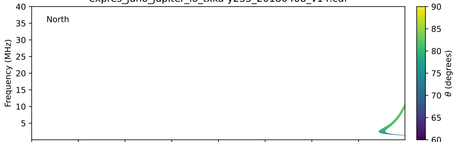
expres_juno_jupiter_io_txka-y235_20180408_v14.cdf
