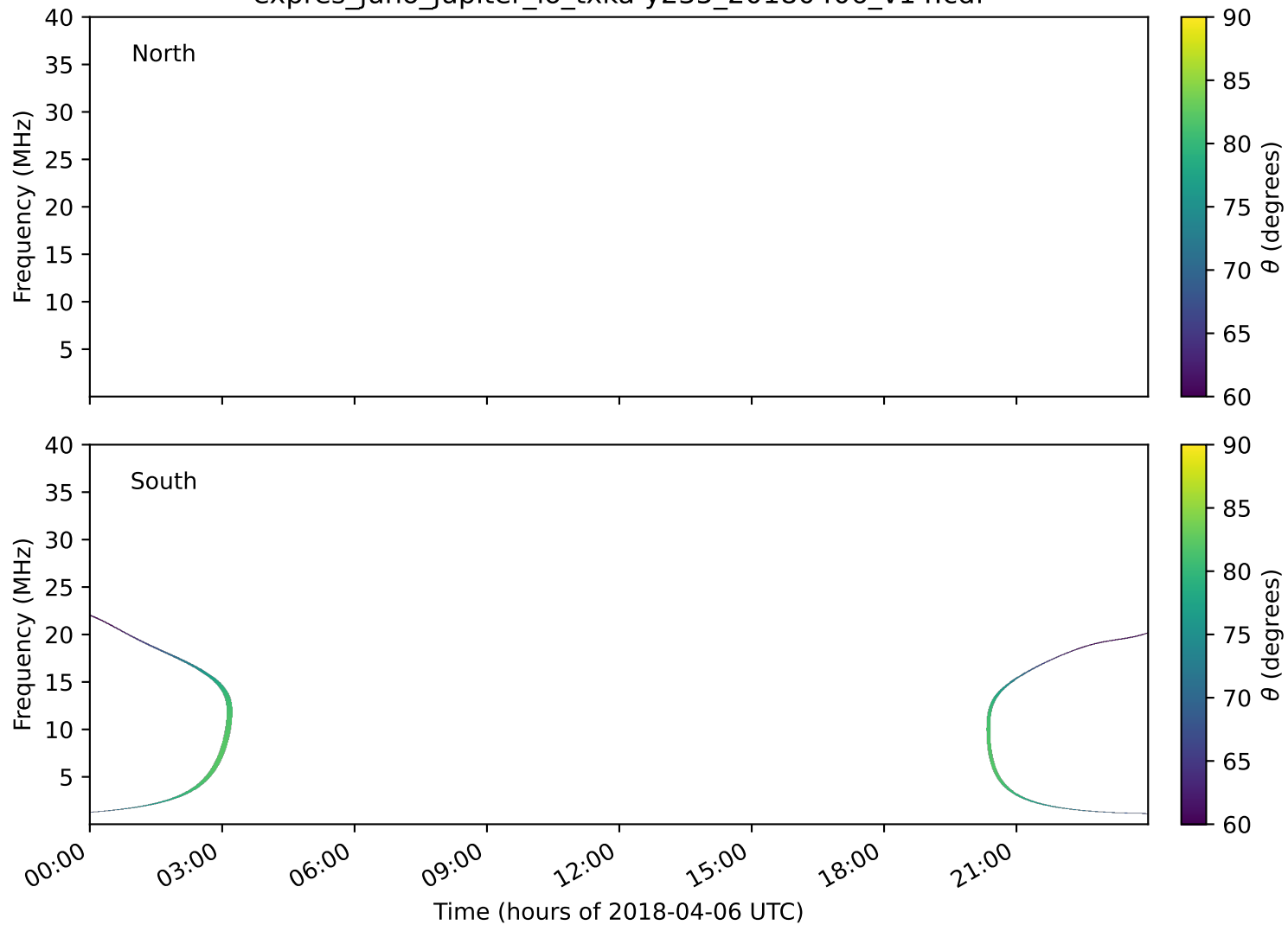
expres_juno_jupiter_io_txka-y235_20180406_v14.cdf
