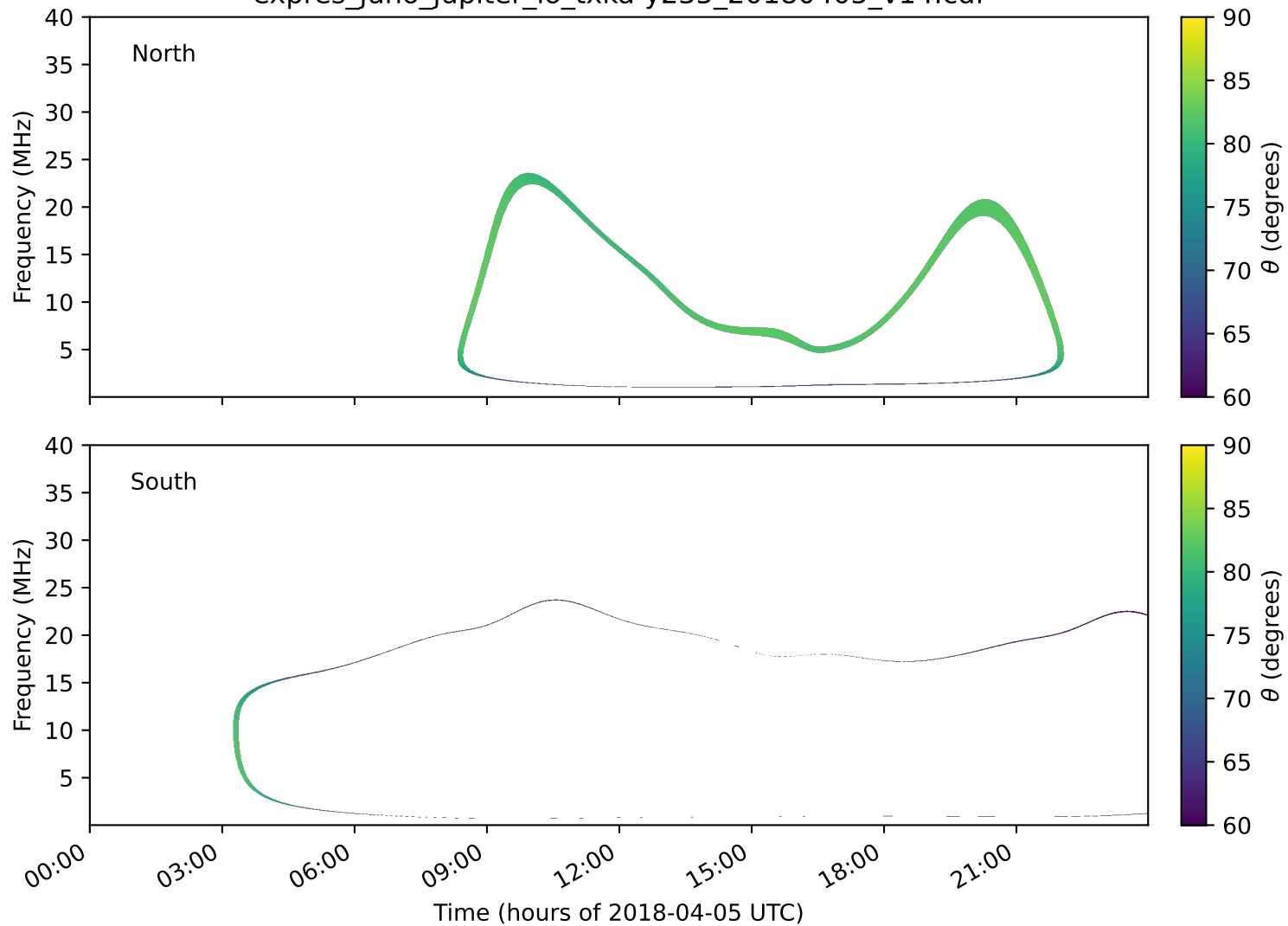
expres_juno_jupiter_io_txka-y235_20180405_v14.cdf
