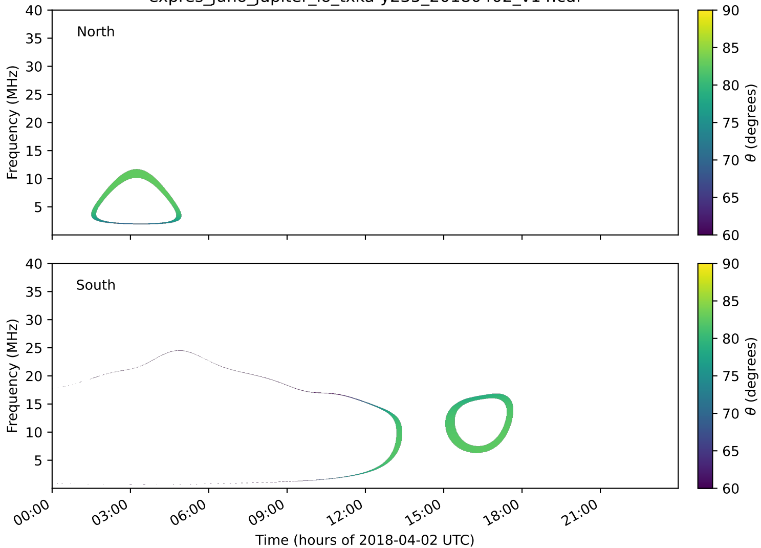
expres_juno_jupiter_io_txka-y235_20180402_v14.cdf
