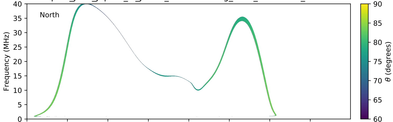
expres_juno_jupiter_io_jrm09_lossc-wid1deg_3kev_20180430_v01.cdf
