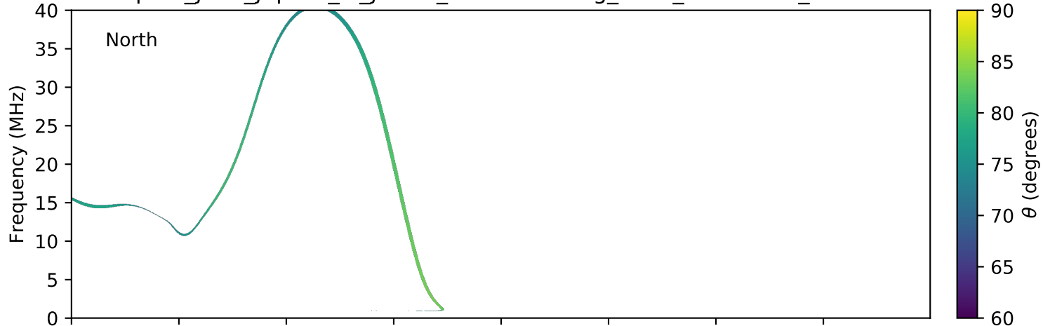
expres_juno_jupiter_io_jrm09_lossc-wid1deg_3kev_20180425_v01.cdf
