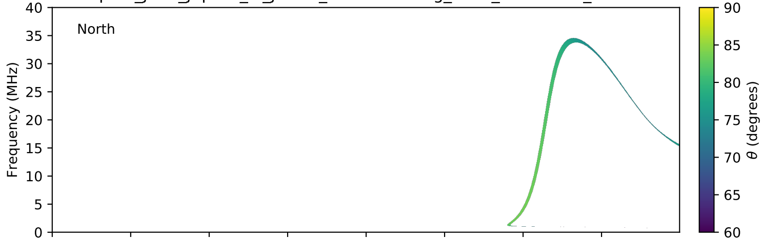
expres_juno_jupiter_io_jrm09_lossc-wid1deg_3kev_20180424_v01.cdf
