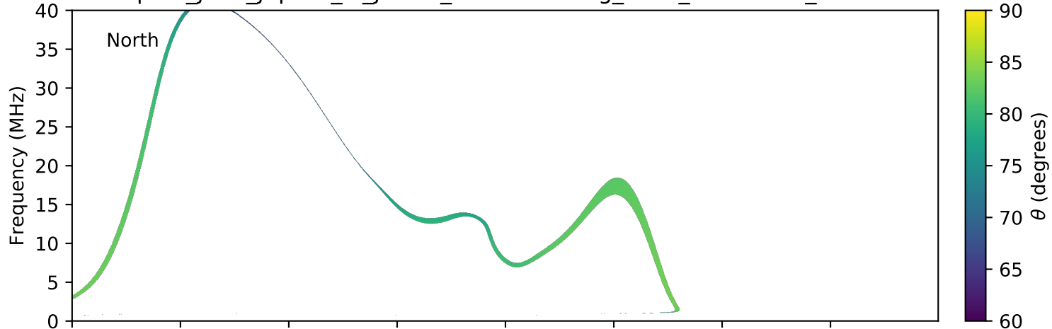
expres_juno_jupiter_io_jrm09_lossc-wid1deg_3kev_20180423_v01.cdf
