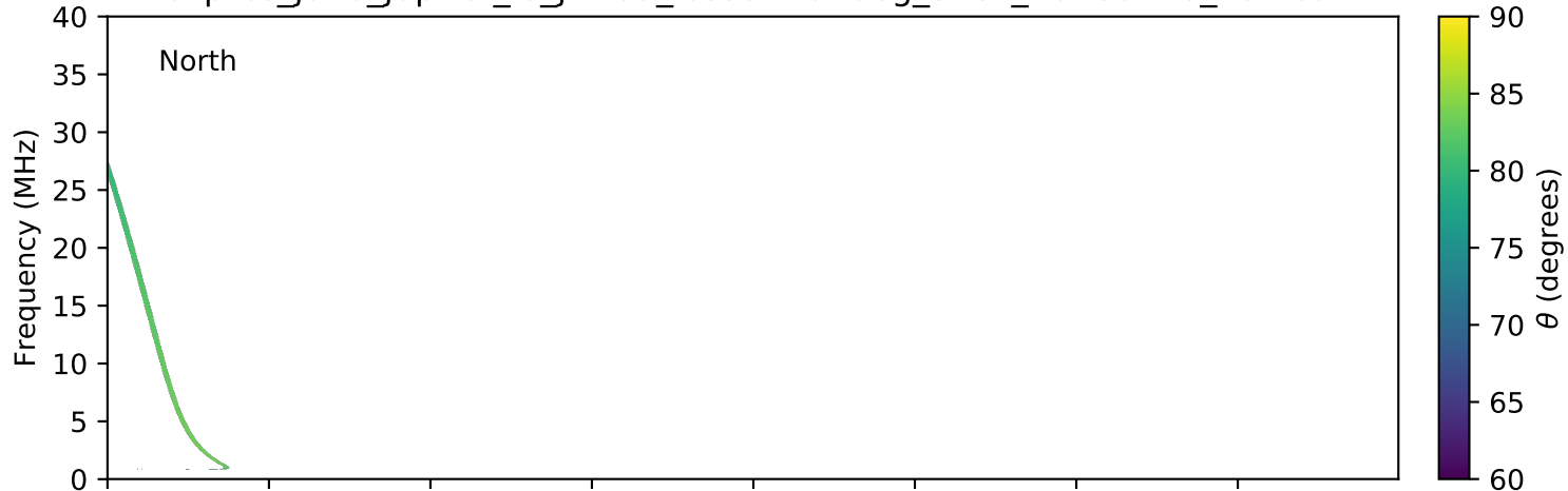
expres_juno_jupiter_io_jrm09_lossc-wid1deg_3kev_20180420_v01.cdf
