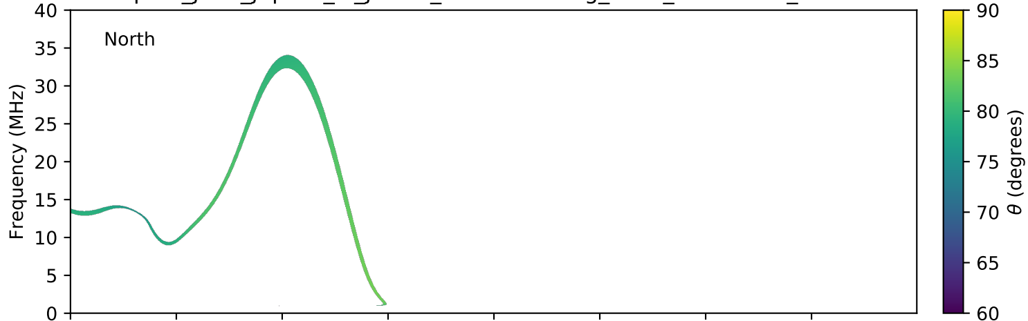
expres_juno_jupiter_io_jrm09_lossc-wid1deg_3kev_20180418_v01.cdf
