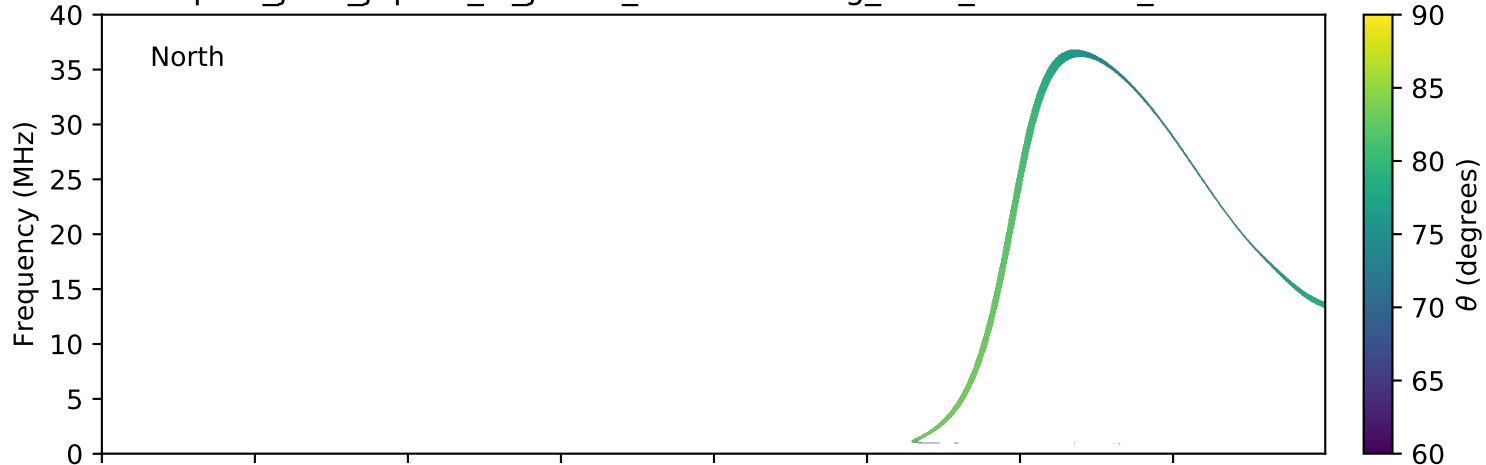
expres_juno_jupiter_io_jrm09_lossc-wid1deg_3kev_20180417_v01.cdf
