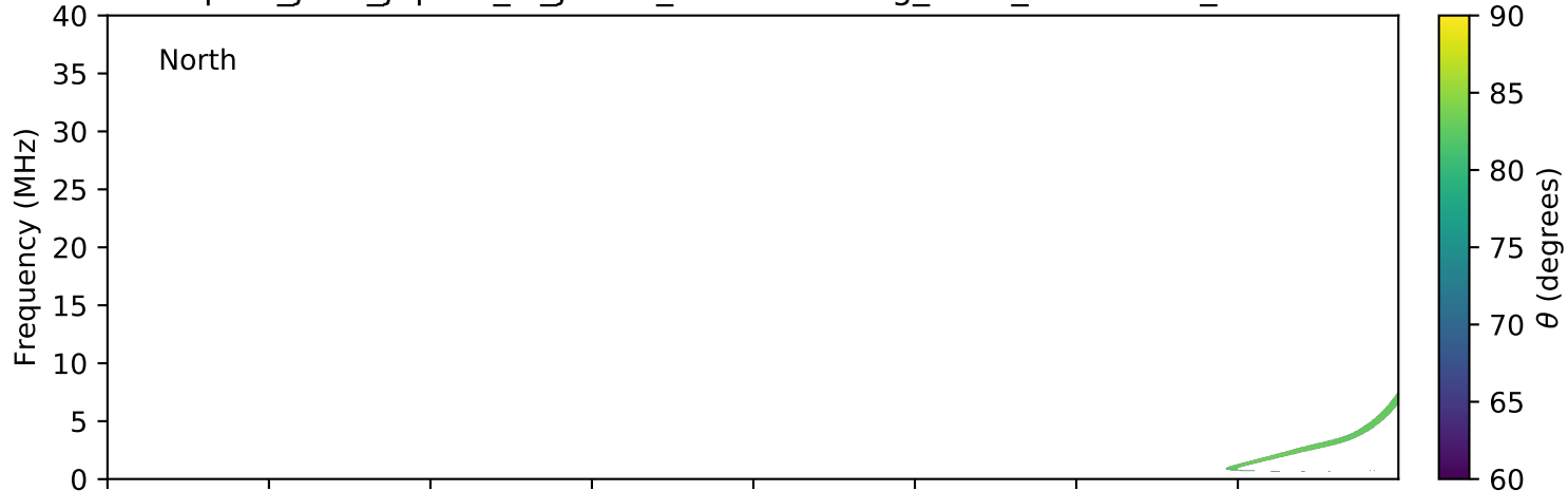
expres_juno_jupiter_io_jrm09_lossc-wid1deg_3kev_20180415_v01.cdf
