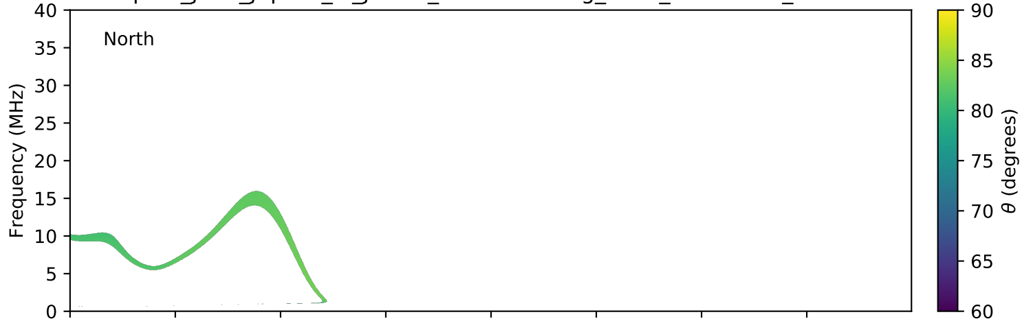
expres_juno_jupiter_io_jrm09_lossc-wid1deg_3kev_20180411_v01.cdf
