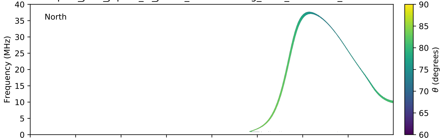
expres_juno_jupiter_io_jrm09_lossc-wid1deg_3kev_20180410_v01.cdf
