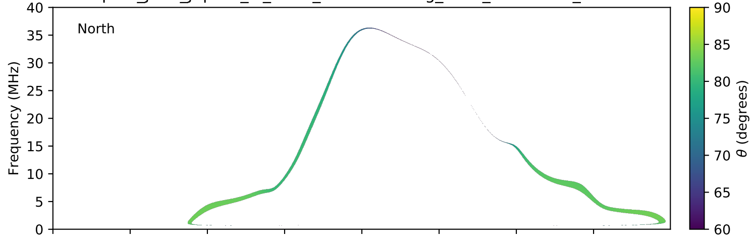
expres_juno_jupiter_io_isaac_lossc-wid1deg_3kev_20180428_v01.cdf
