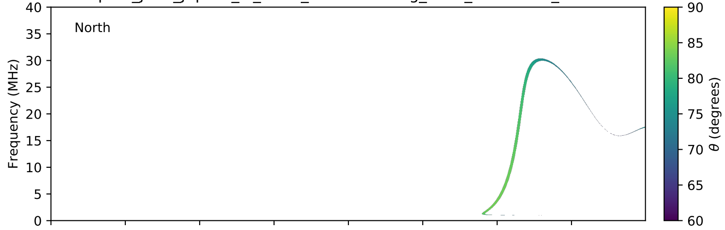
expres_juno_jupiter_io_isaac_lossc-wid1deg_3kev_20180424_v01.cdf
