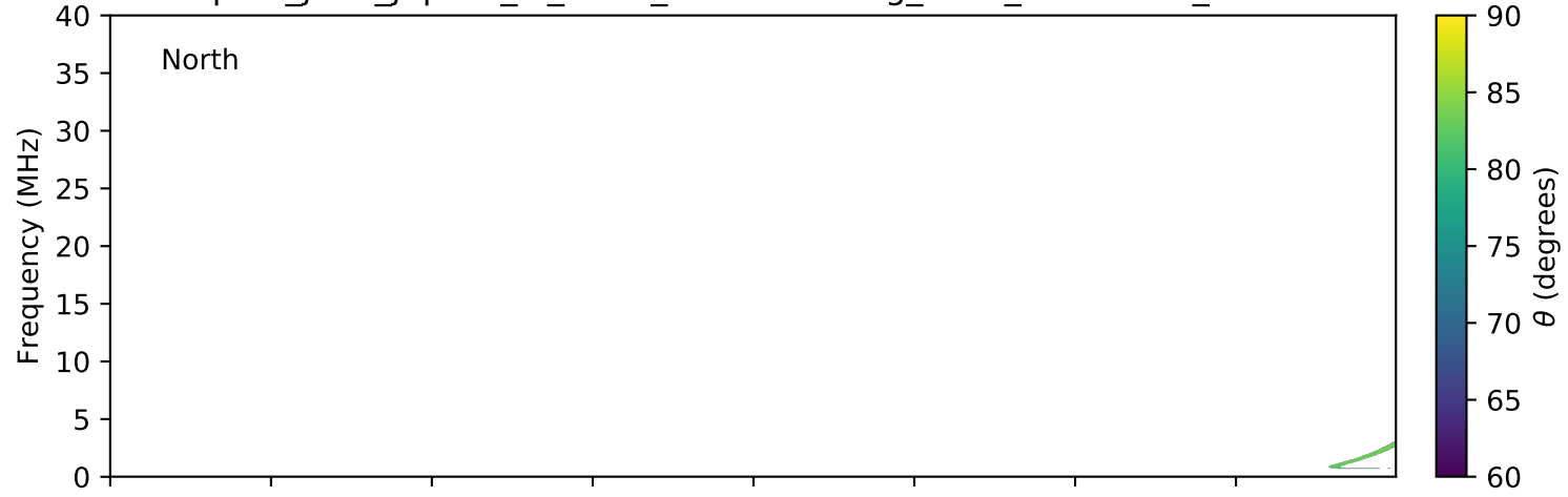
expres_juno_jupiter_io_isaac_lossc-wid1deg_3kev_20180422_v01.cdf
