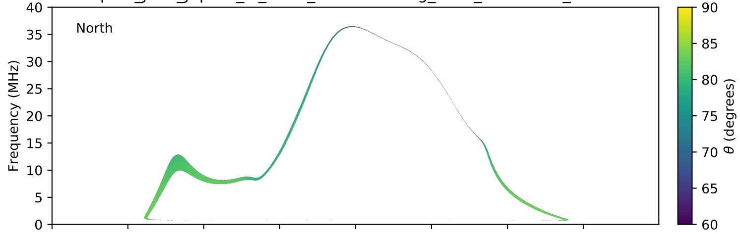
expres_juno_jupiter_io_isaac_lossc-wid1deg_3kev_20180421_v01.cdf
