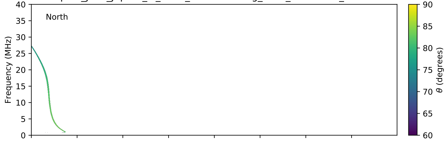
expres_juno_jupiter_io_isaac_lossc-wid1deg_3kev_20180420_v01.cdf
