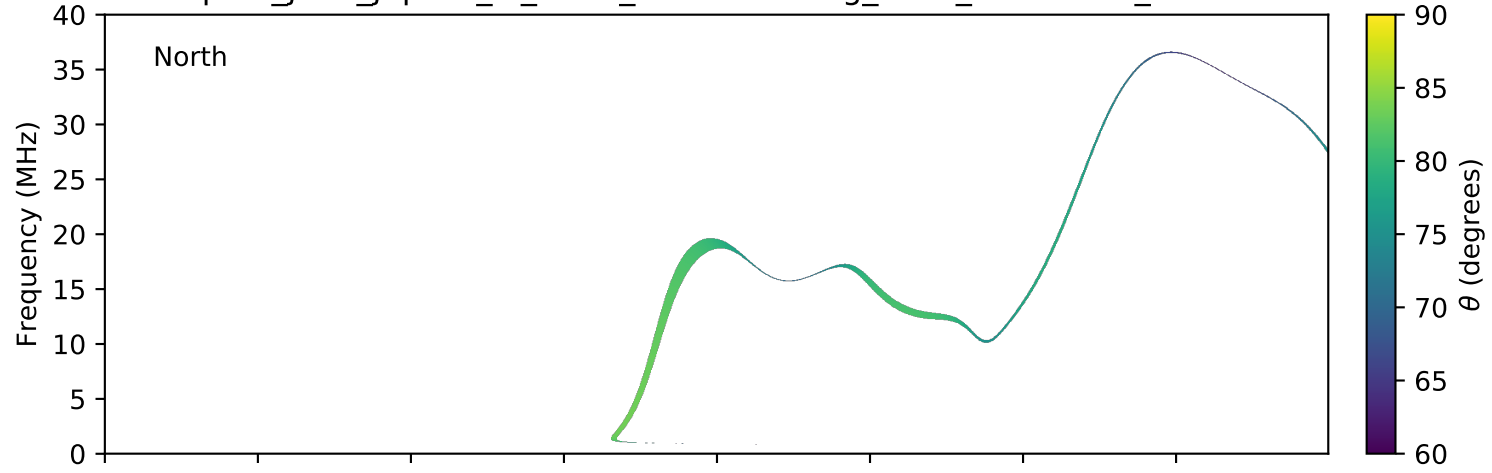
expres_juno_jupiter_io_isaac_lossc-wid1deg_3kev_20180419_v01.cdf
