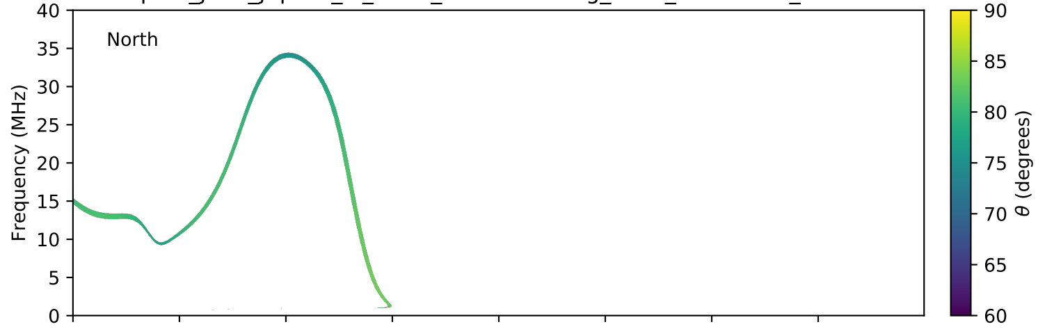
expres_juno_jupiter_io_isaac_lossc-wid1deg_3kev_20180418_v01.cdf
