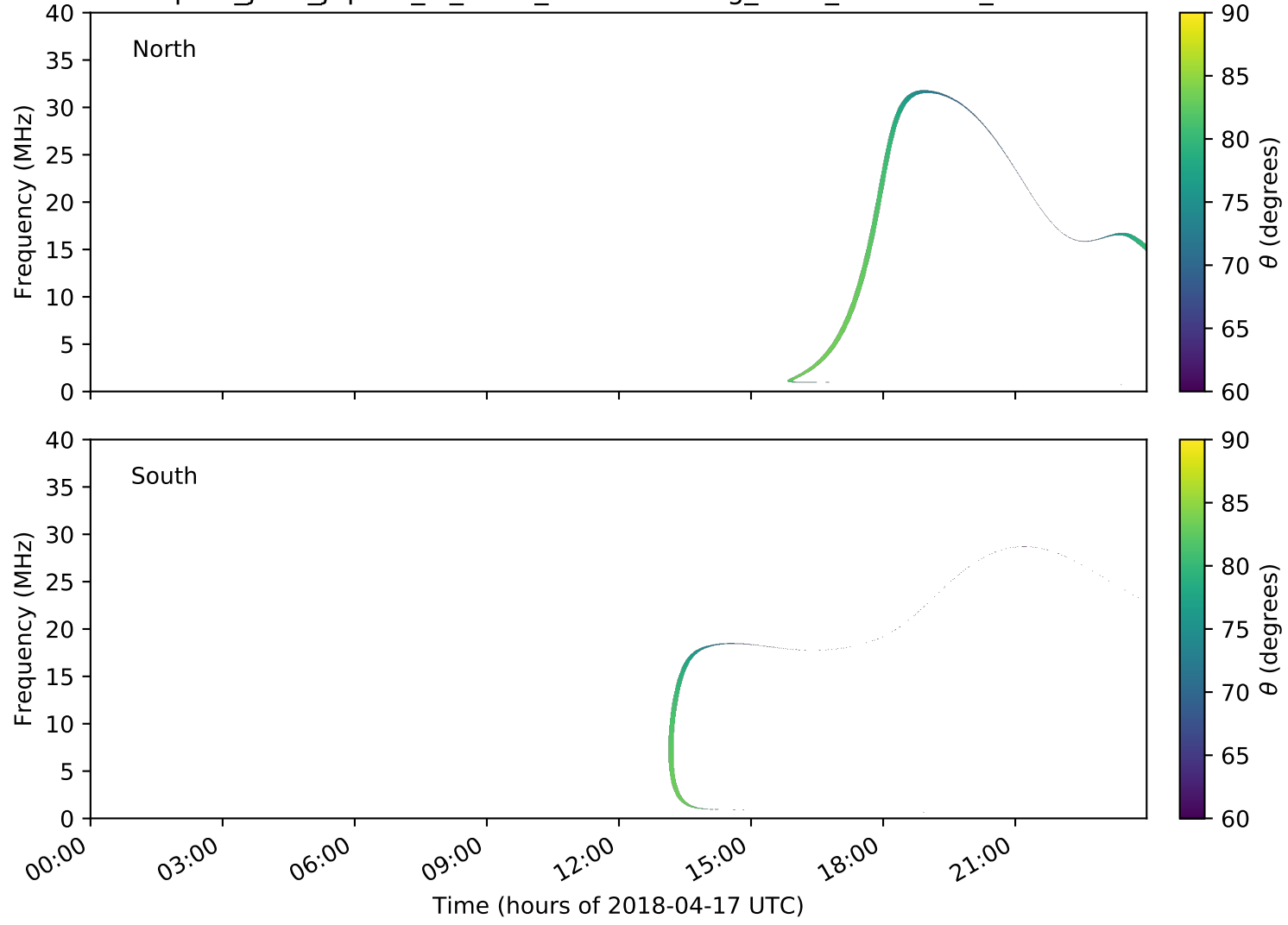
expres_juno_jupiter_io_isaac_lossc-wid1deg_3kev_20180417_v01.cdf
